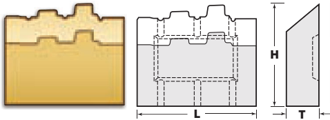
3/4-BUCA SET EXTRA TALL W/COOLANT GROOVE 517-8073/517-8083/517-8093
