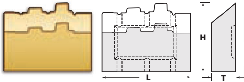
3/4-BUCA SET – COOLANT GROOVE 517-8075/517-8085/517-8095
